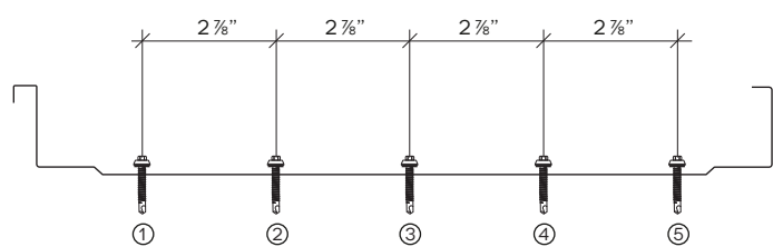
TYPICAL SCREW SEQUENCE AT VALLEY
