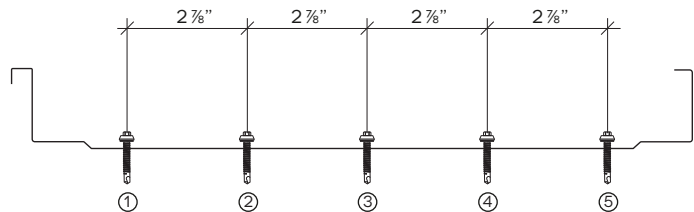
TYPICAL SCREW SEQUENCE AT EAVE
