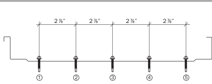
TYPICAL SCREW SEQUENCE AT EAVE
