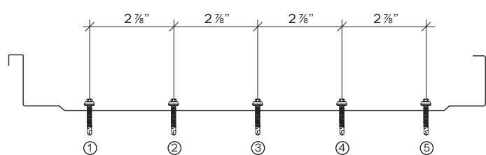
TYPICAL SCREW SEQUENCE AT HIGH EAVE
